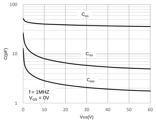
Figure 10: Capacitance Characteristics
