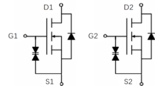
Schematic Diagram
