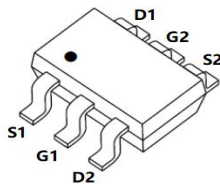
SOT-363-6L (Dual) top view
